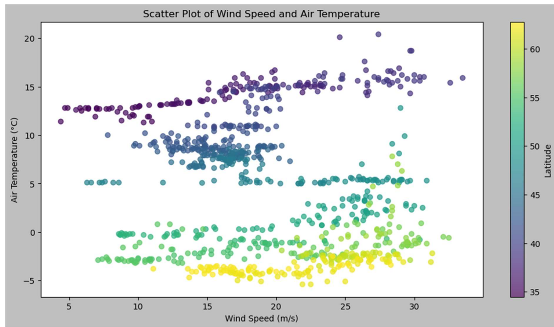
Figure 4: Scatter plot showcasing air temperature (°C) and wind speed (m/s) across latitudes from 35° to 60° and above.
