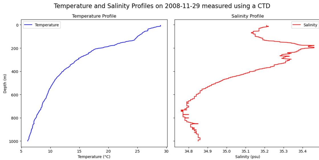
Figure 1: Line graphs displaying the temperature and salinity profile measured using a CTD.
