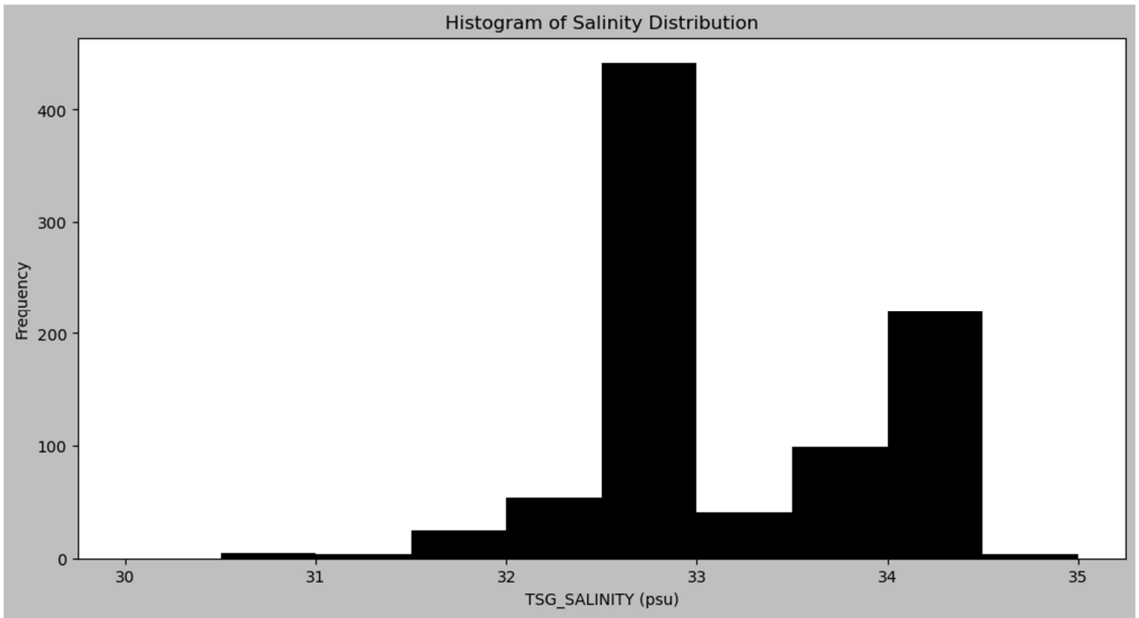
Figure 3: Histogram displaying the frequencies of sea surface salinity (psu) that was measured with a TSG ((Thermosalinograph). The data collected every ten minutes starting from the departure time at 17:10pm on the 28/06/2017 and ending on the 23:50pm on the 04/07/2017. The data was collected whilst aboard the SA Agulhas II.
