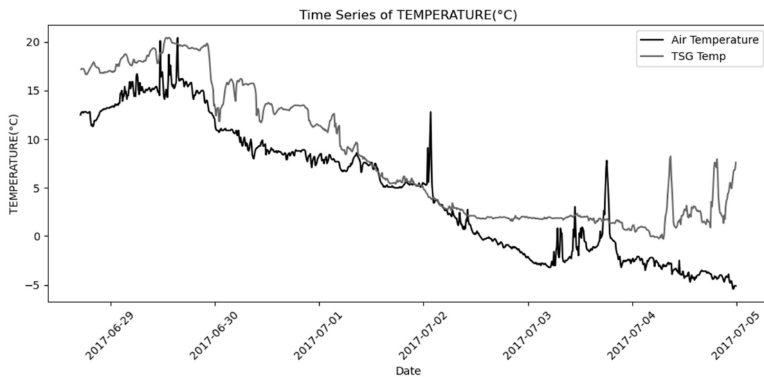
Figure 2: Line graph displaying the temperatures (°C) taken roughly every 10 minutes from 17:10pm to 23:50 between the 28/06/2017 to the 04/07/2017. These measurements were collected aboard the South African Agulhas II vessel. The temperatures measured and displayed include both air temperature as well as sea surface temperature.
