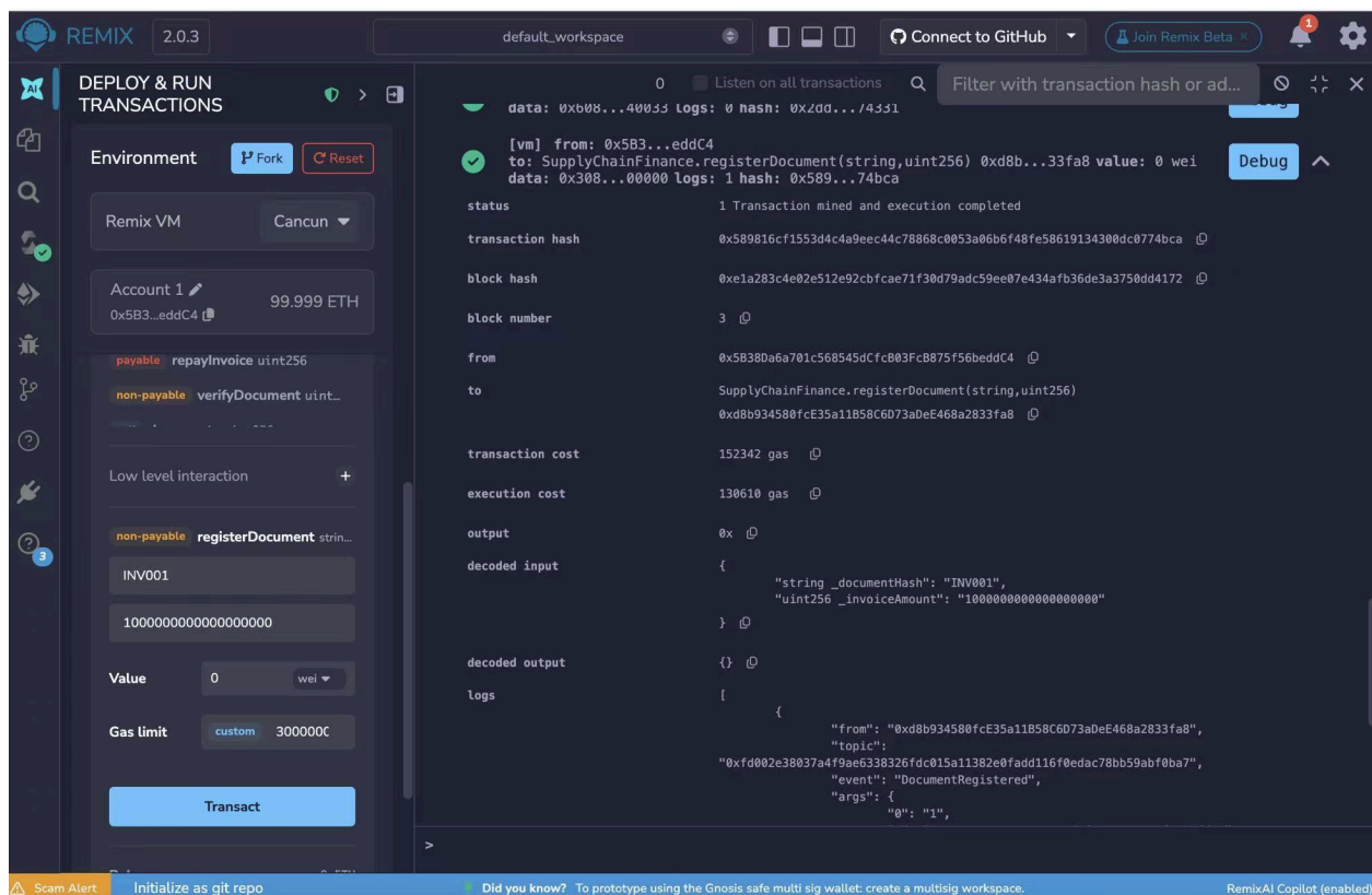
Figure 1: Register Document
