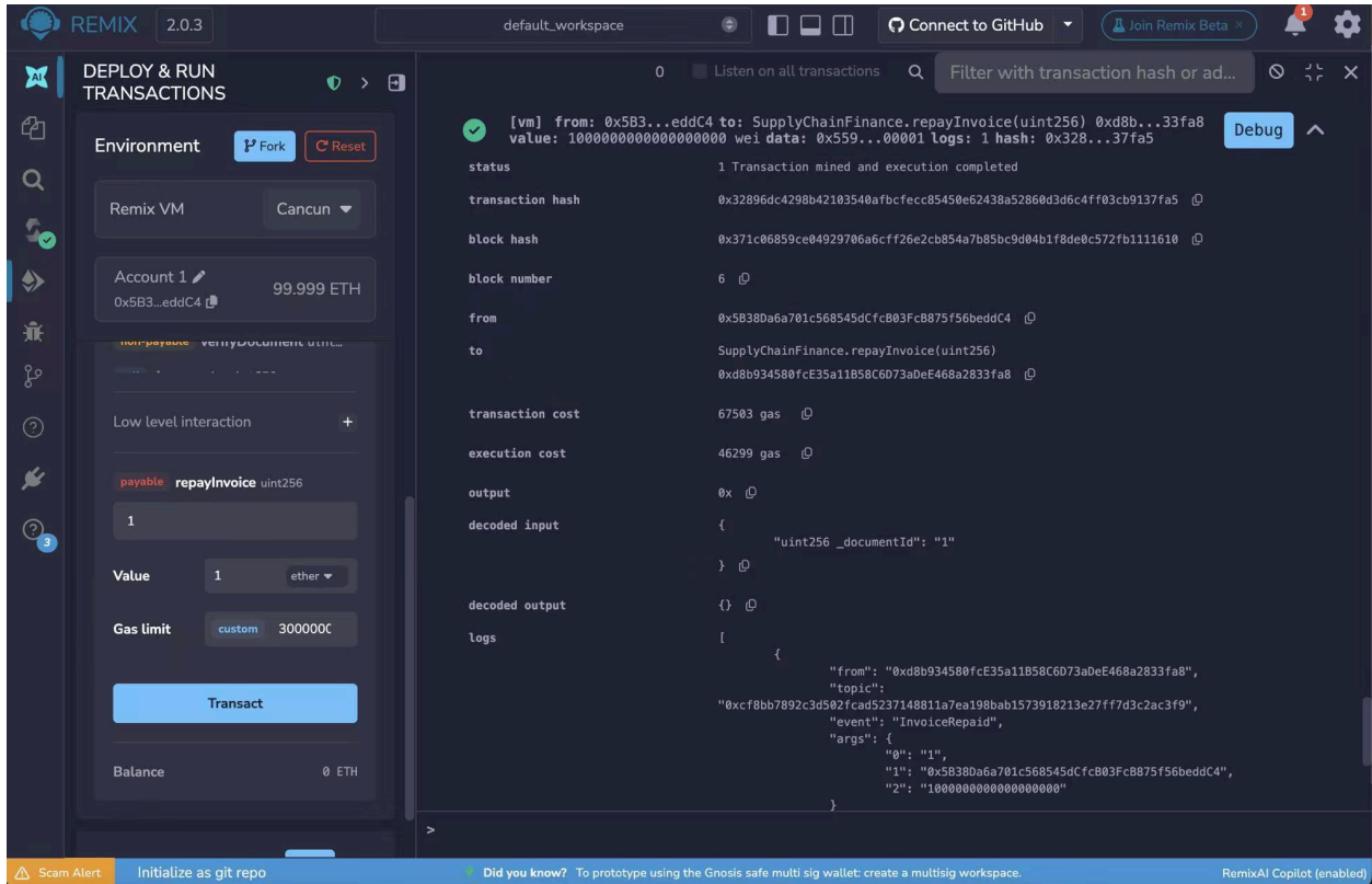
Figure 4: Repay Invoice
