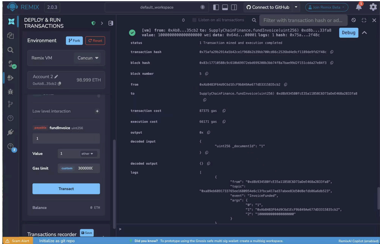
Figure 3: Fund Invoice
