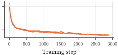
U-Net, 12 bands
