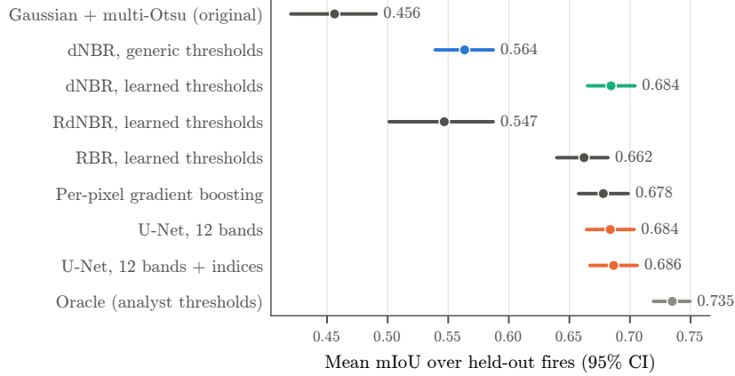
Figure 3: Calibrated dNBR and both U-Nets reach the same accuracy, and the analyst-threshold oracle is higher. Mean mIoU over the 31 held-out fires with 95% bootstrap confidence intervals from resampling fires.
