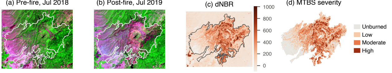
Figure 1: The task on the 2018 Camp Fire. (a, b) Landsat surface reflectance before and after the fire (SWIR2, NIR, and red composite), from the scenes named in the MTBS record. (c) dNBR computed from the two scenes. (d) The MTBS severity map, produced by an analyst who chose dNBR thresholds for this fire. The white or gray line is the MTBS fire perimeter, and only pixels inside it are labeled. A method sees (a) and (b) and must predict (d).
