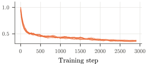
U-Net, 12 bands + indices
