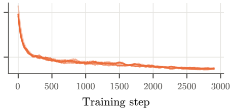
U-Net, 12 bands
