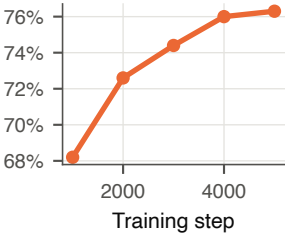
Severity accuracy
