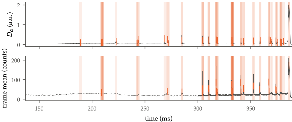
shot 27305: 40 D_\alpha spikes, 31 camera spikes
