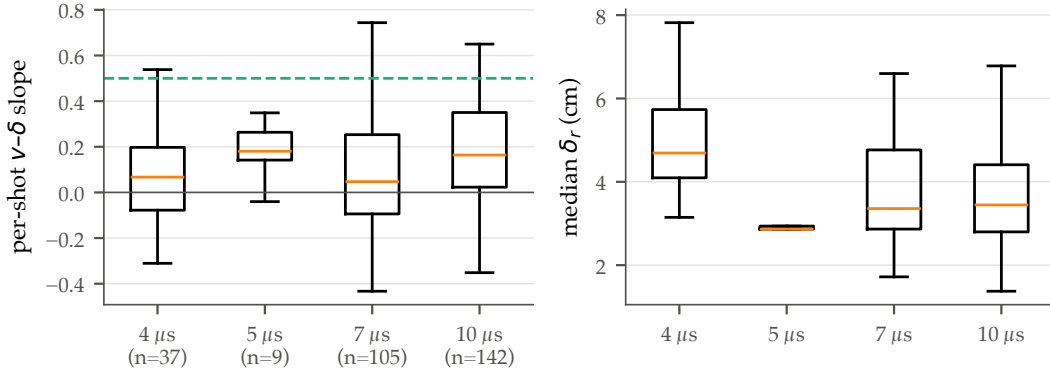
Figure 5: Effect of exposure time. Left: per-discharge velocity–width slopes by exposure setting; the dashed line is the inertial scaling. Right: per-discharge median width by exposure.
