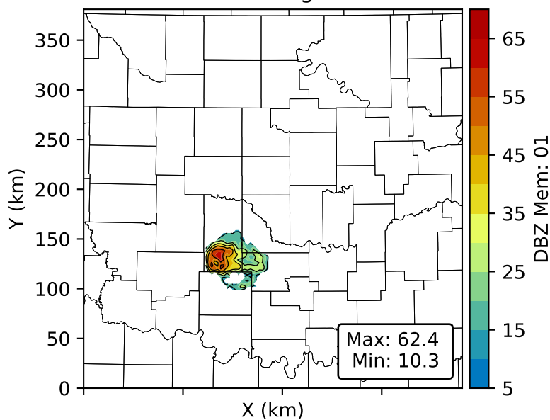
DBZ Mem: 01 Height: 0.72 km
