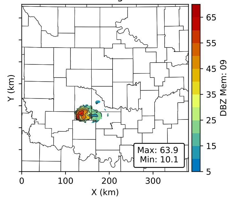
DBZ Mem: 09 Height: 0.72 km
