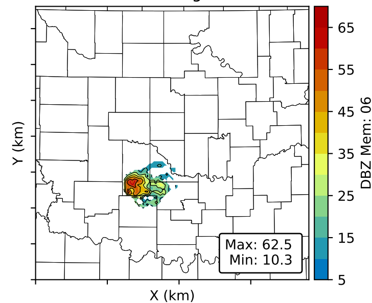
DBZ Mem: 06 Height: 0.72 km
