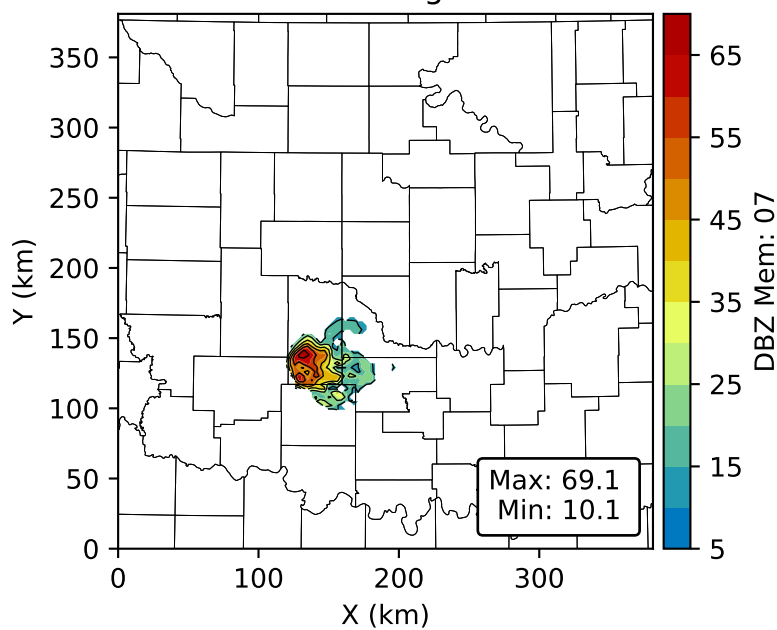
DBZ Mem: 07 Height: 0.72 km
