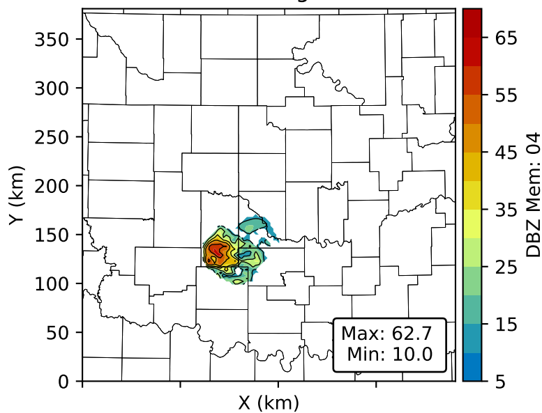
DBZ Mem: 04 Height: 0.72 km
