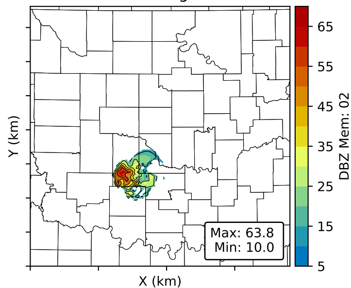
DBZ Mem: 02 Height: 0.72 km
