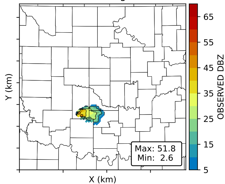
OBSERVED DBZ Height: 0.90 km
