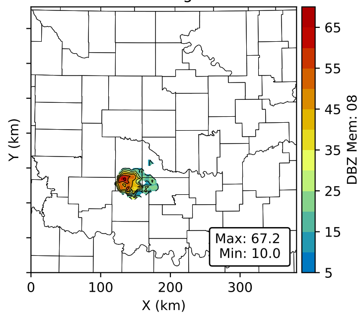
DBZ Mem: 08 Height: 0.72 km
