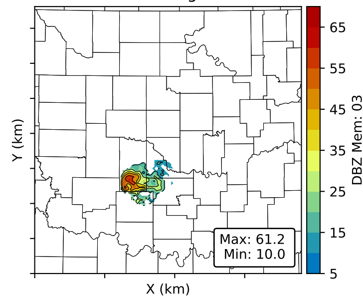
DBZ Mem: 03 Height: 0.72 km
