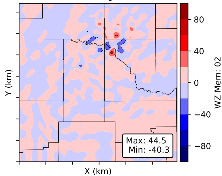
WZ Mem: 02 Height: 0.72 km
