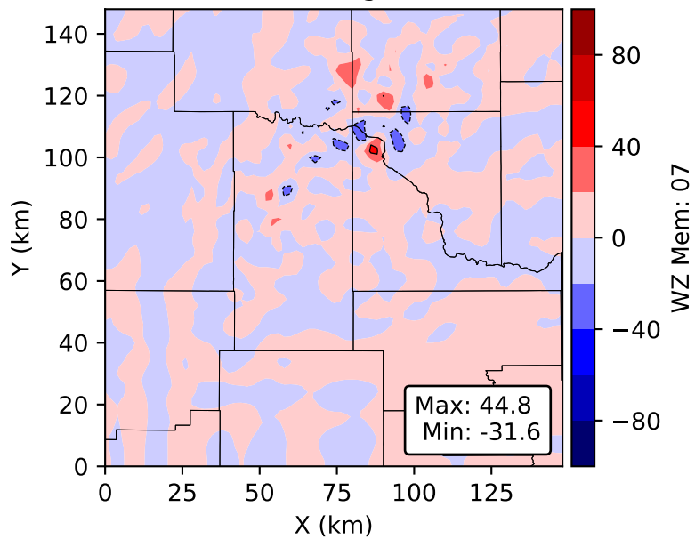
WZ Mem: 07 Height: 0.72 km
