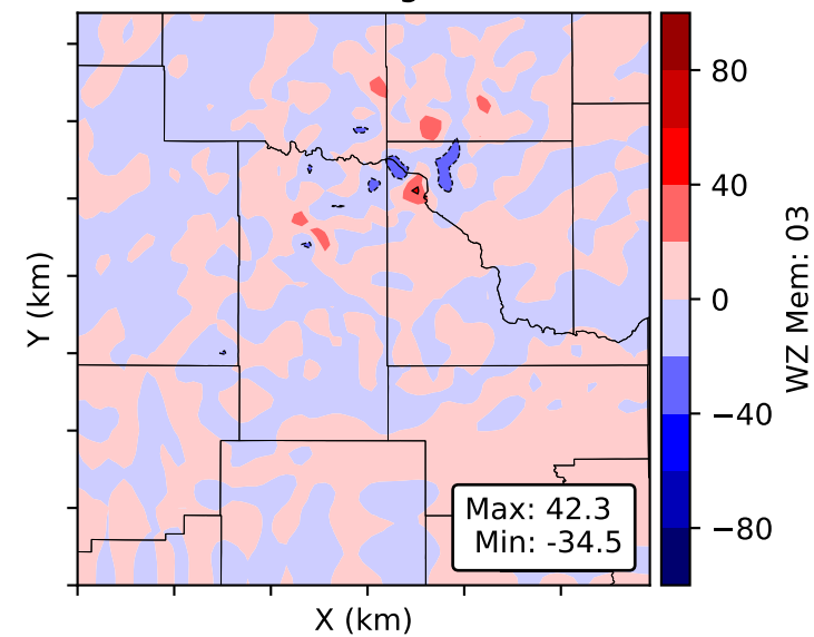
WZ Mem: 03 Height: 0.72 km
