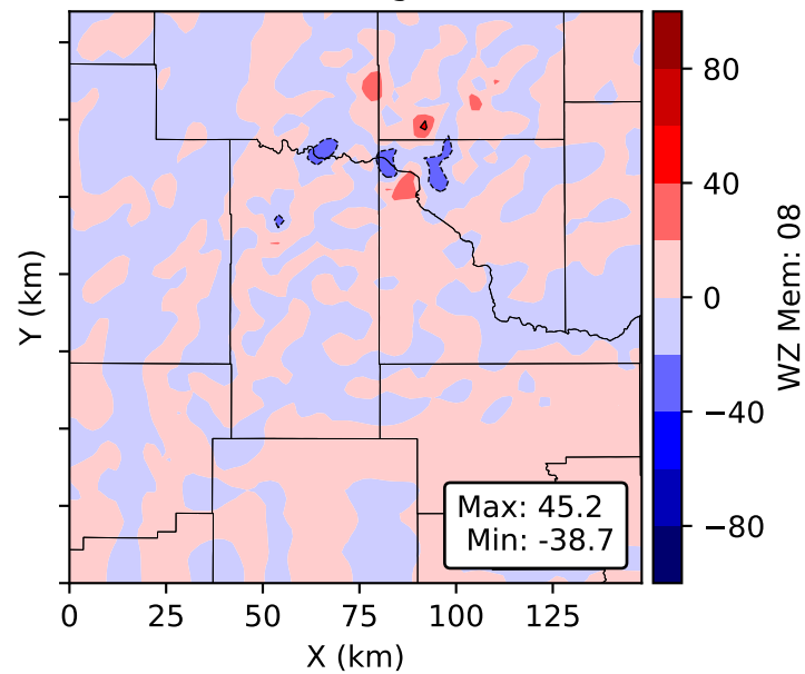
WZ Mem: 08 Height: 0.72 km
