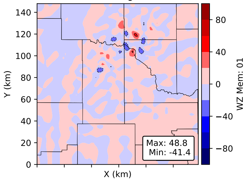
WZ Mem: 01 Height: 0.72 km
