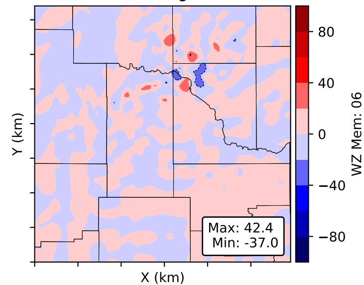
WZ Mem: 06 Height: 0.72 km
