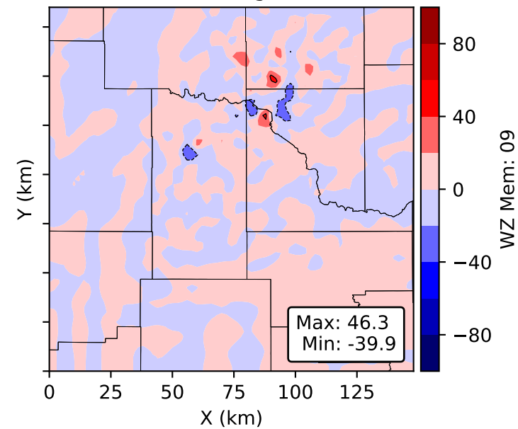
WZ Mem: 09 Height: 0.72 km
