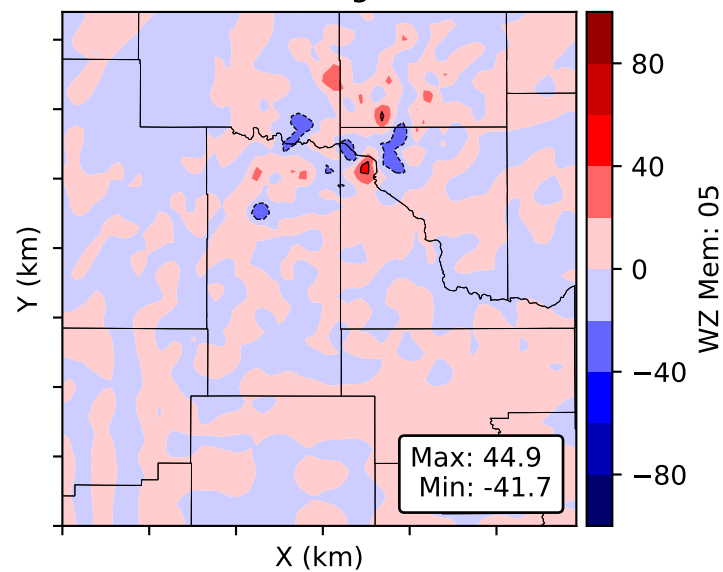
WZ Mem: 05 Height: 0.72 km
