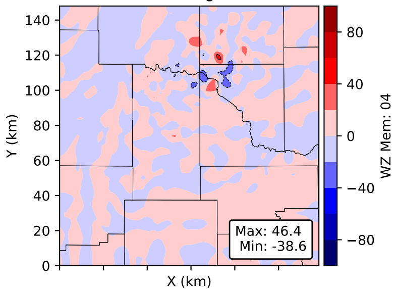
WZ Mem: 04 Height: 0.72 km
