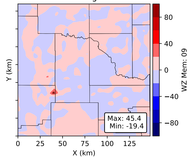
WZ Mem: 09 Height: 0.75 km
