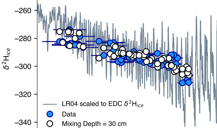
b. MOT simulation with LR04 scaled to EDC
