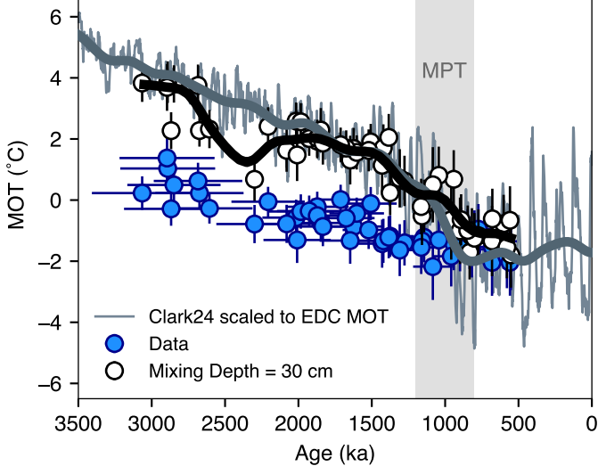
c. MOT simulation with Clark24 scaled to EDC
