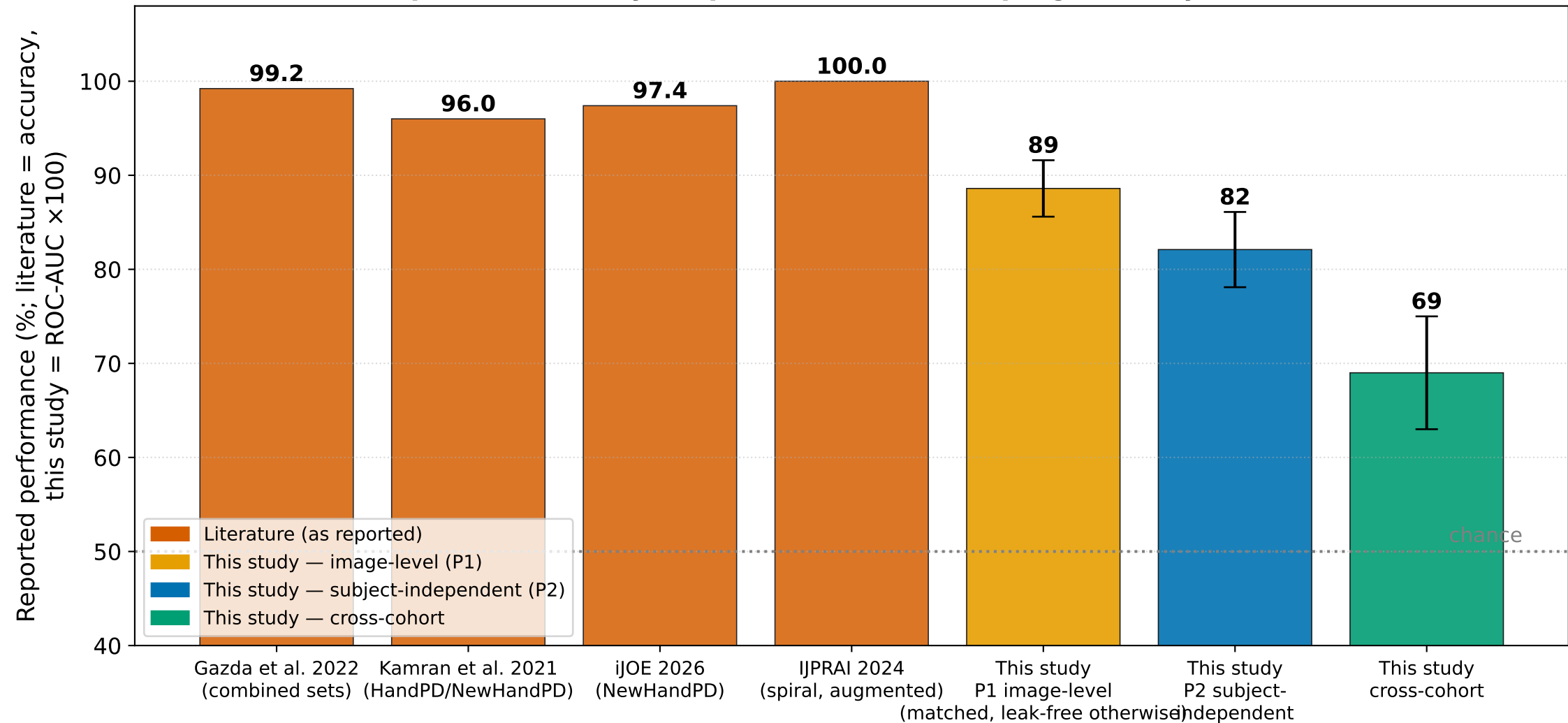
Literature-reported accuracy vs. performance under progressively stricter evaluation
