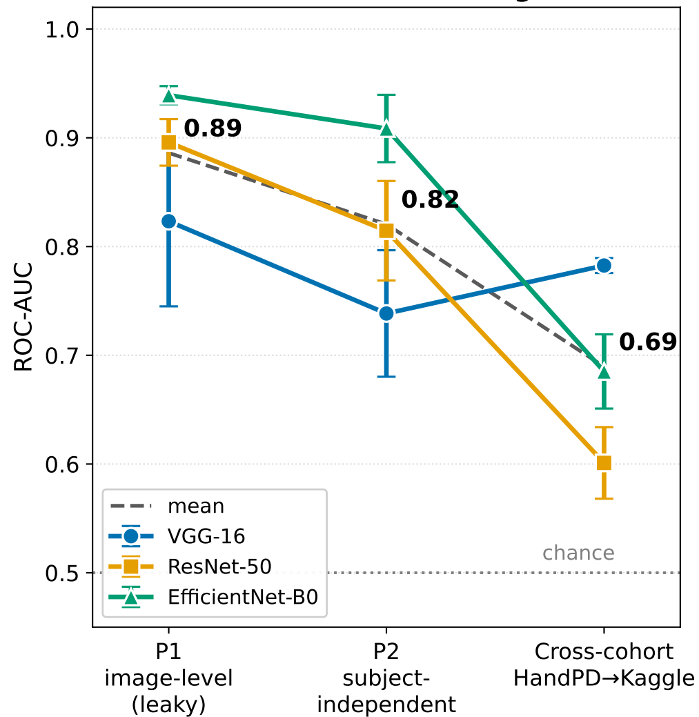
(a) Discrimination falls as leakage is removed
