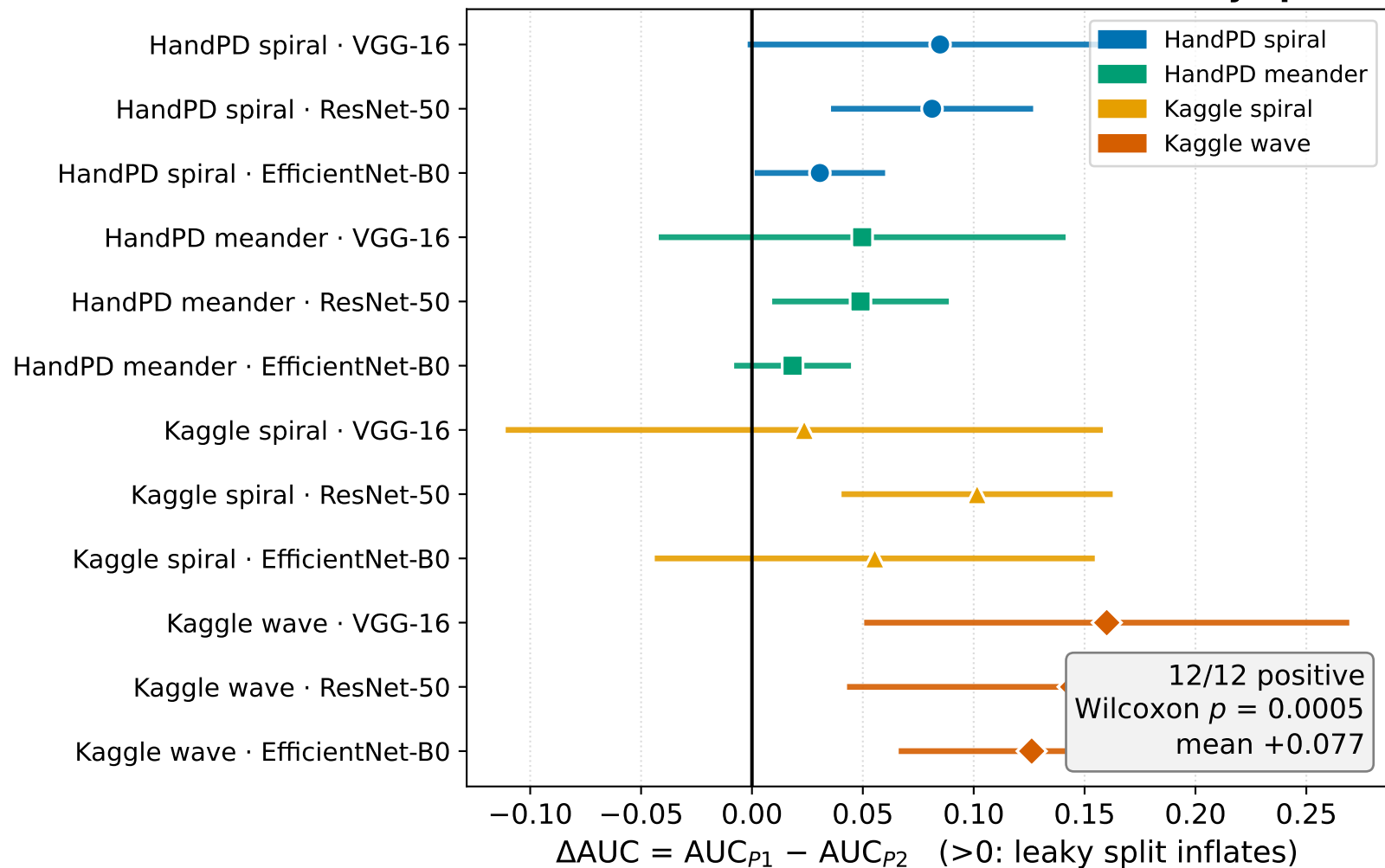
(b) All 12 combinations favour the leaky split
