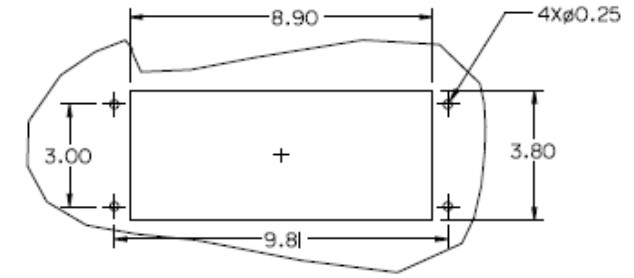
DETAIL A SCALE 0.250
