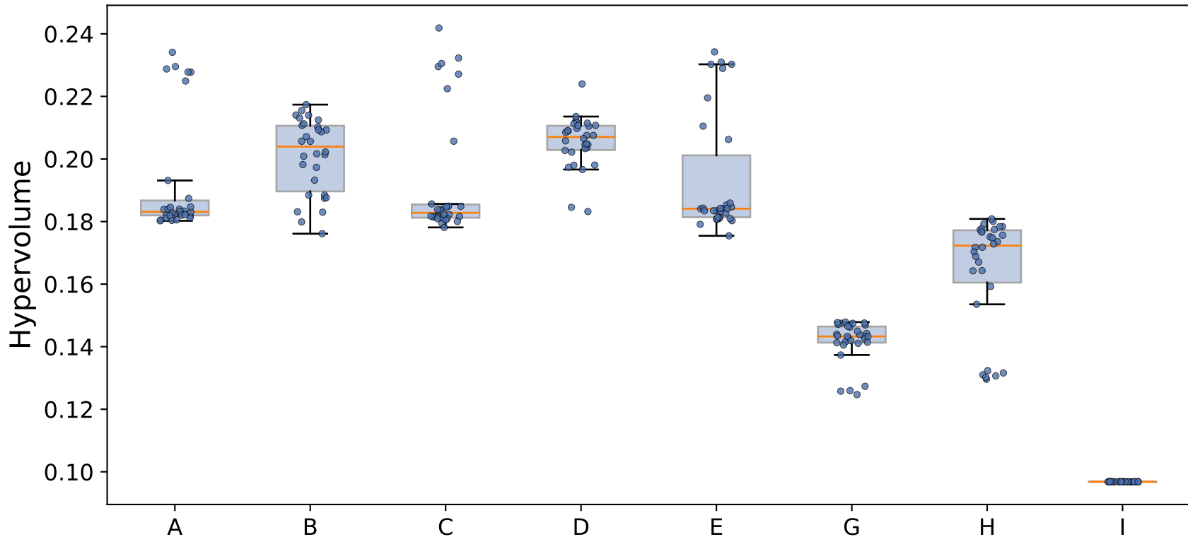
Decoder ablation (8 variants, 30 seeds)
