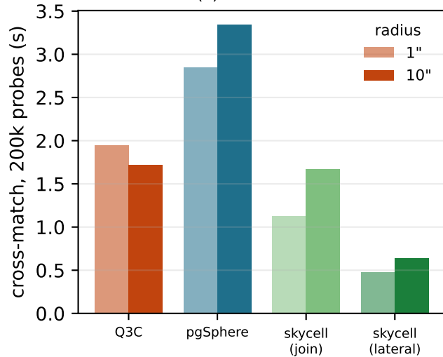
(c) cross-match
