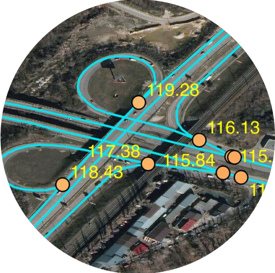
Figure 2. Representation of elevated road structures in the network model. Nodes are depicted as orange points, and road segments (edges) are shown as neon blue lines. Node elevations, expressed in meters relative to local mean sea level, are annotated in yellow. The basemap imagery is sourced from Bing Satellite .
