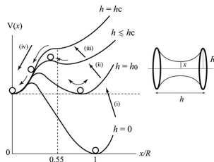
Figure 9. The surface energy V(x) of the soap film for various values of the parameter h . Here x represents the minimum catenoid radius. The circles indicate the positions occupied by the film. Equations (6) correspond to the transitions (i) \rightarrow (ii), (ii) \rightarrow (iii), (iii) \rightarrow (iv).
