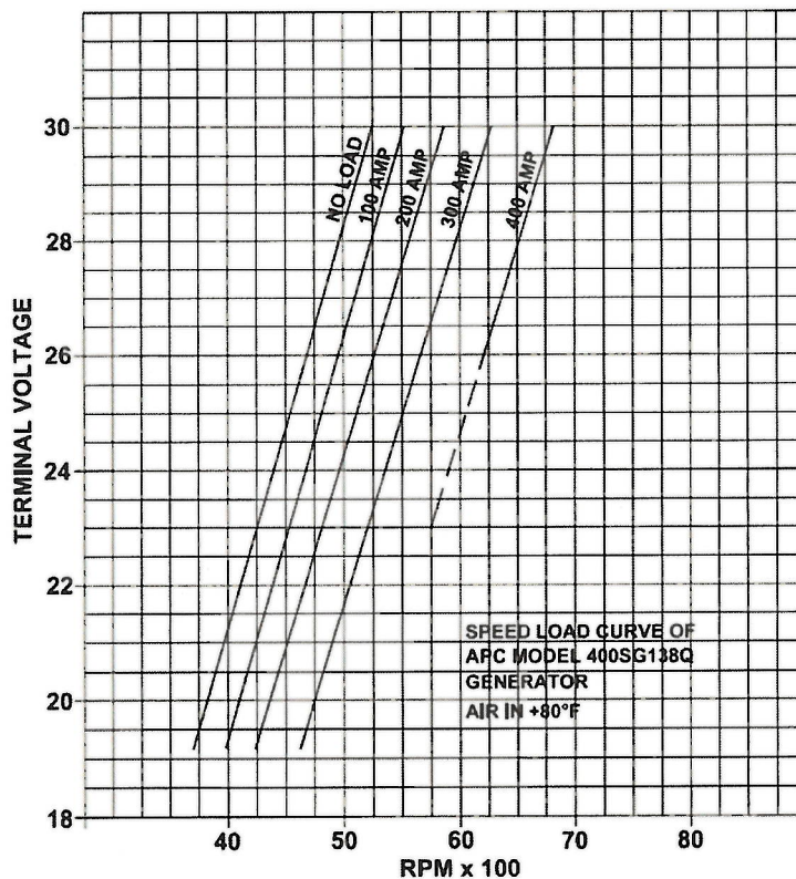
SPEED-LOAD CURVE
