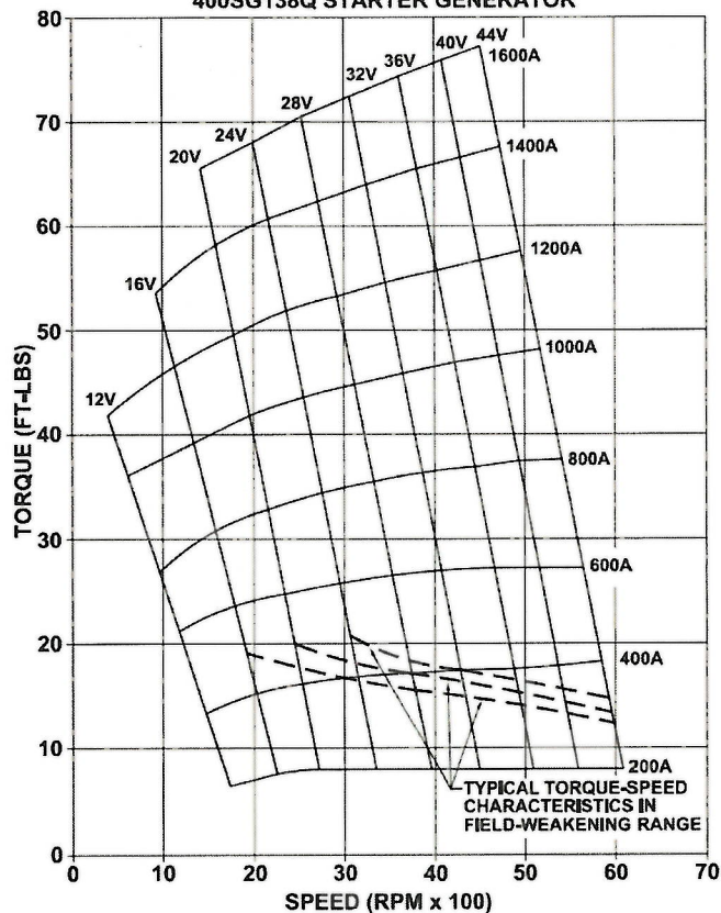
SPEED-TORQUE CURVE 400SG138Q STARTER GENERATOR
