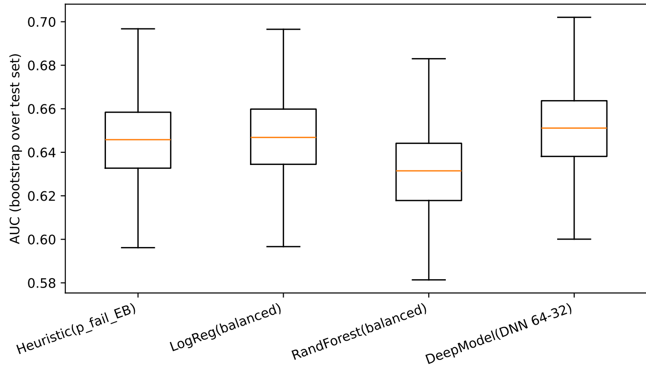
Model Comparison: AUC Distribution (Bootstrap)
