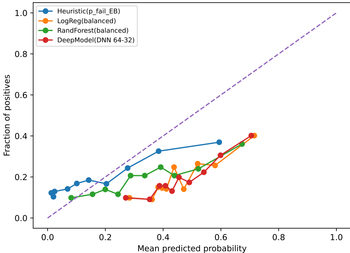
Calibration Curves (Test Month)
