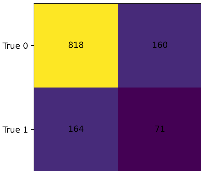
RandomForest(balanced) thr=0.47
