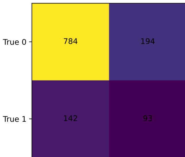
DeepModel(DNN 64-32) thr=0.55
