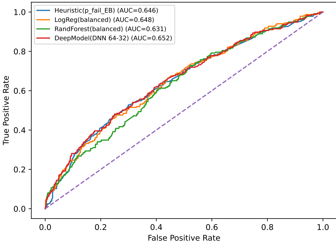
ROC Curves (Test Month)
