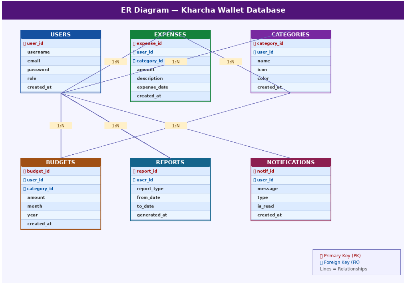
Figure 5.1 — ER Diagram: Kharcha Wallet Database Schema (PK = Primary Key, FK = Foreign Key)
