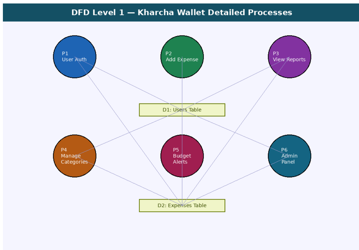
Figure 4.2 — DFD Level 1: Detailed Process Decomposition
