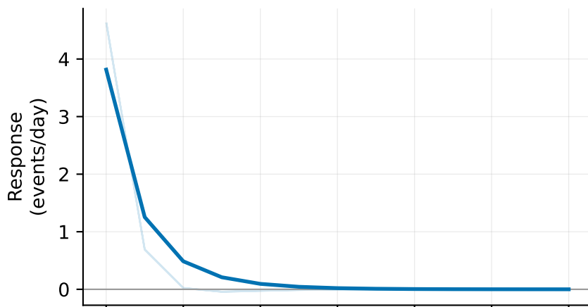
US/Israeli strikes shock → US/Israeli strikes
