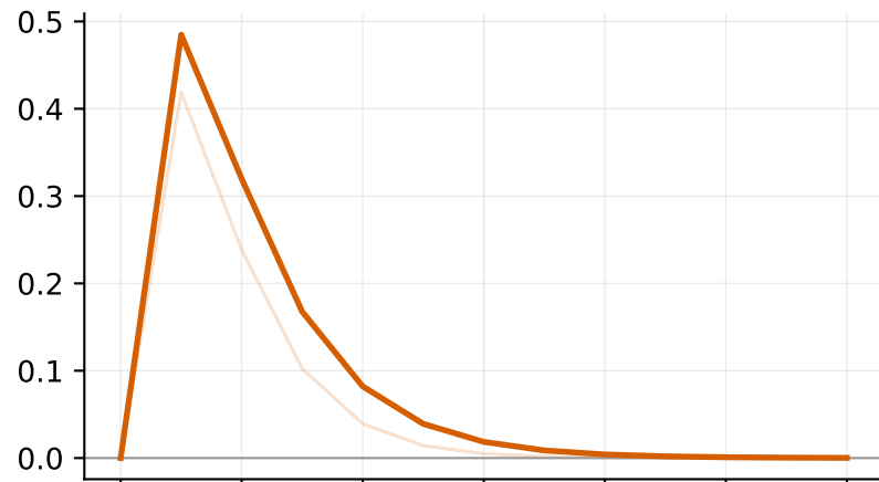
Iranian retaliation shock → US/Israeli strikes
