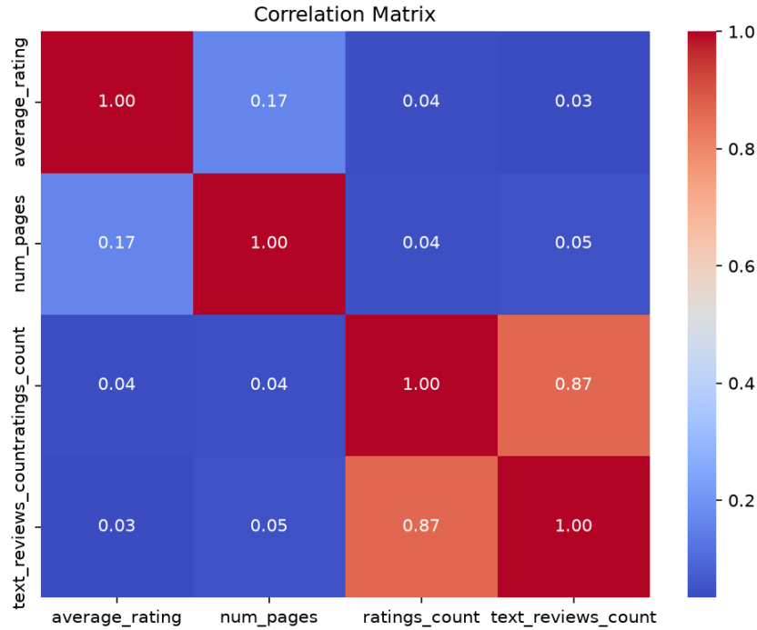
Figure 1: Correlation matrix of original numeric features.
