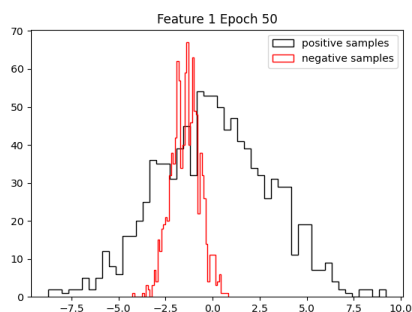
feature_1
