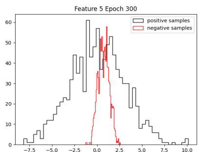
feature_5
