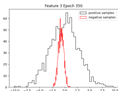
feature_3
