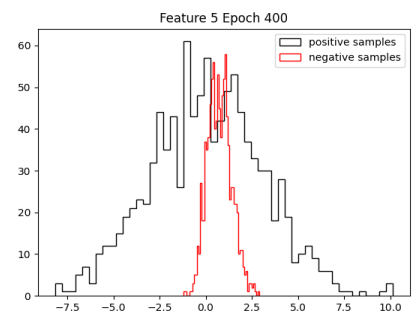
feature_5
