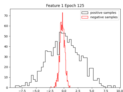
feature_1
