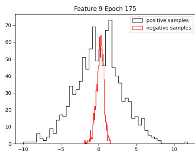
feature_9
