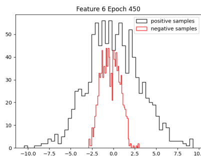
feature_6
