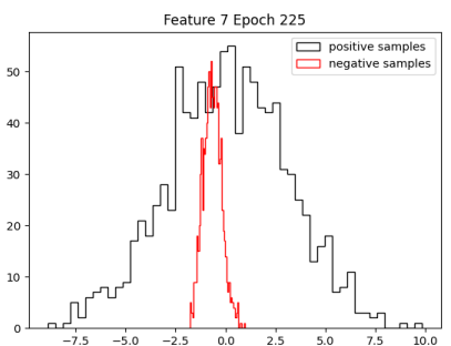
feature_7
