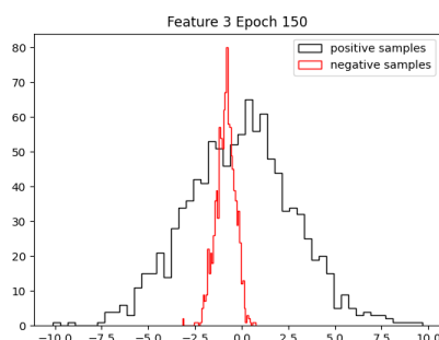
feature_3
