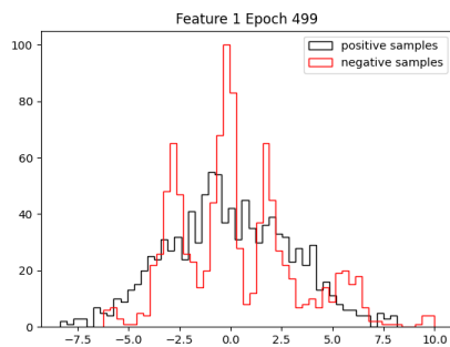
feature_1
