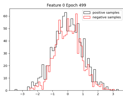
feature_0
