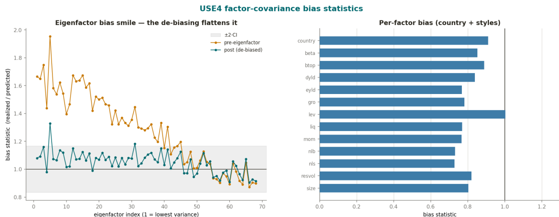
Figure 1: The eigenfactor bias, before and after de-biasing, over the monthly backtest. Left: the bias statistic b_k = \text{realized/predicted risk} across the eigenfactors, ordered from lowest to highest variance. Before the adjustment the lowest-variance eigenfactors realize up to \approx 1.95\times their predicted risk while the highest-variance ones are mildly over-predicted ( b < 1 ) – the downward “smile” of a too-dispersed spectrum – and after the Monte-Carlo de-biasing the whole curve flattens into the \pm 2 ·CI band around one. Right: the per-factor bias for the country and style factors, all close to one (mildly conservative). The mean absolute deviation |b - 1| falls from \approx 0.31 to \approx 0.07 .
