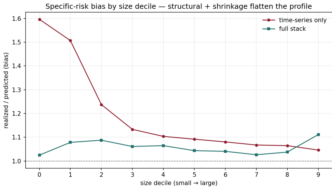
Figure 1: Specific-risk bias (realized / predicted) by size decile, smallest to largest, over the out-of-sample backtest. A time-series-only forecast (the steeply-sloped curve) under-predicts small-cap specific risk badly – bias \approx 1.6 in the smallest decile, falling toward one for large caps – because short, noisy histories and bid–ask bounce understate idiosyncratic risk for small names. The full five-layer stack (the flat curve) holds the profile to \approx 1.0 – 1.1 across all deciles (spread \approx 0.1 , down from > 0.5 ; the two cross only at the very largest decile). The structural and shrinkage layers earn their place exactly where the time series fails.
