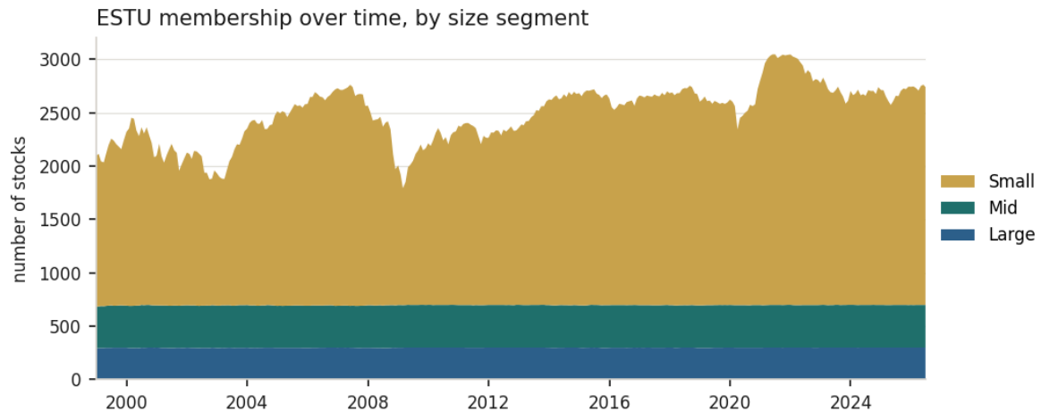
Figure 3: ESTU membership over time, by size segment. Breadth holds near \approx 2,500 names — the MSCI USA IMI scale — dipping in the 2002 and 2008–09 drawdowns as names fail the liquidity and cap screens.
