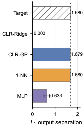
(b) In-sample separation
