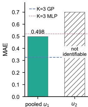
(c) Pooling deletes u_2
