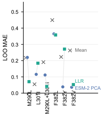
(b) Fixed-feature endpoint errors
