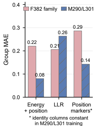
(c) Site-transfer MAE
