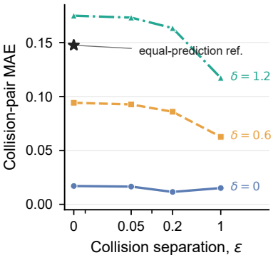
(a) Collision-pair error
