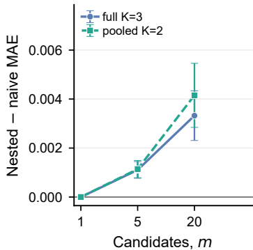
(c) Selection optimism
