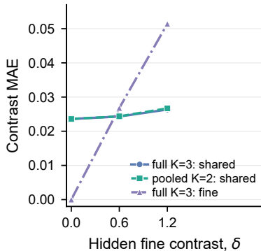
(b) Resolution controls error
