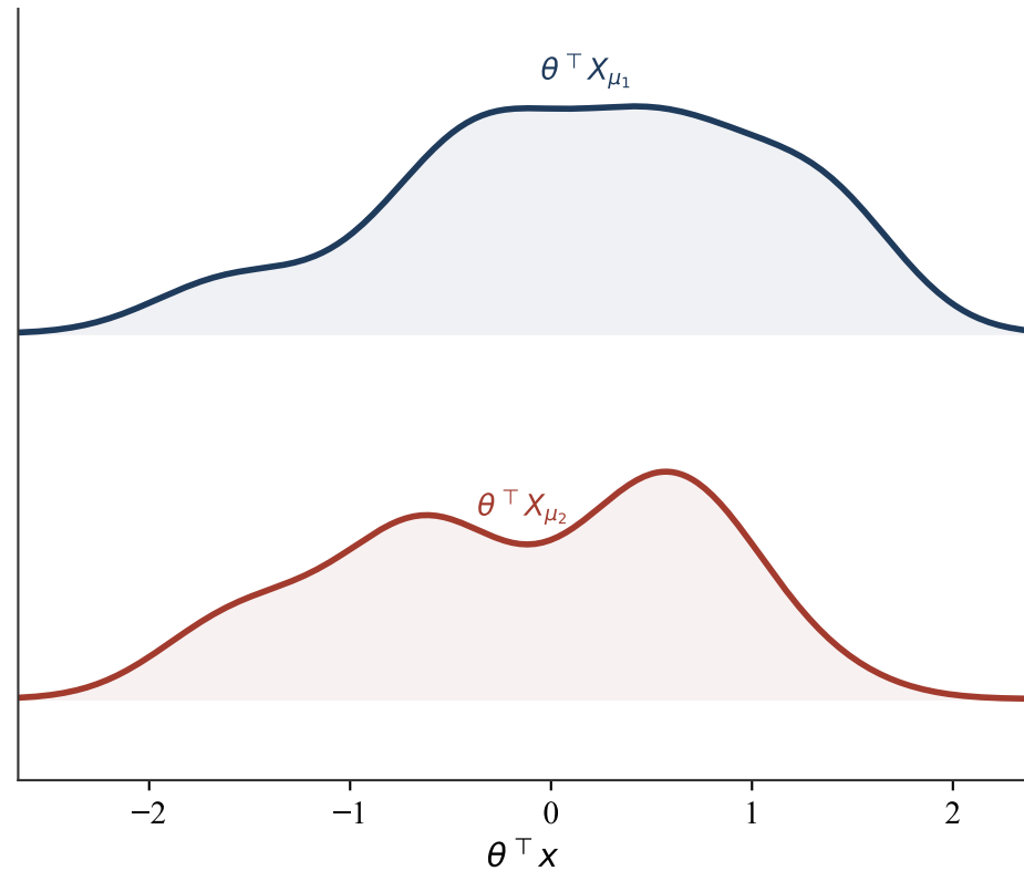
(b) 1D projected distributions — W_2 by sorting quantiles
