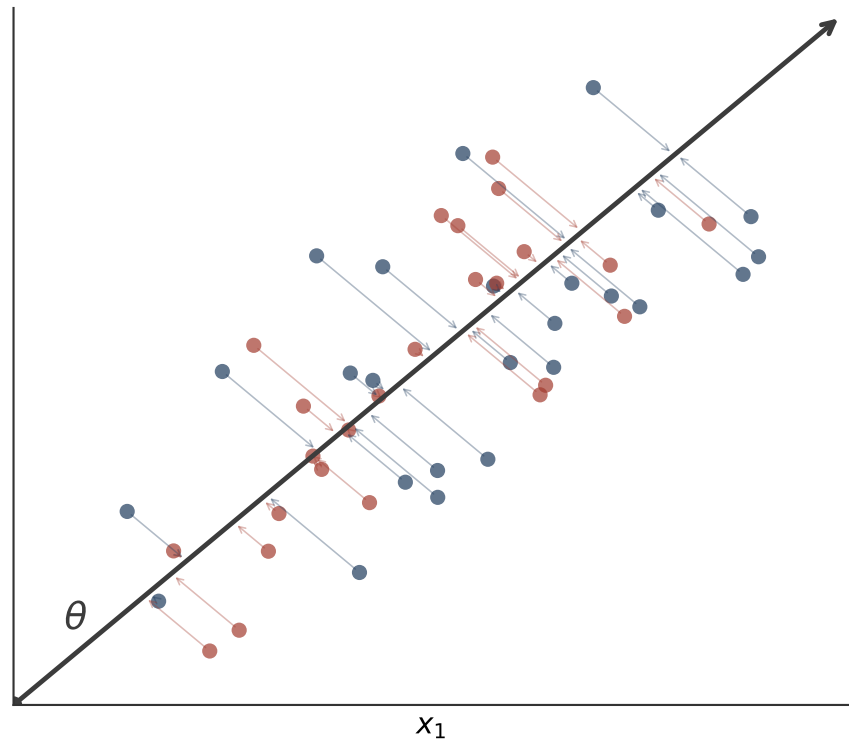
(a) Two distributions in \mathbb{R}^2 — projection onto \theta
