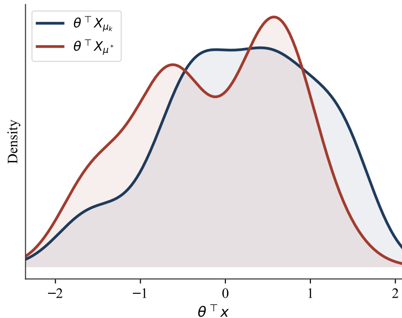
(a) Projected densities
