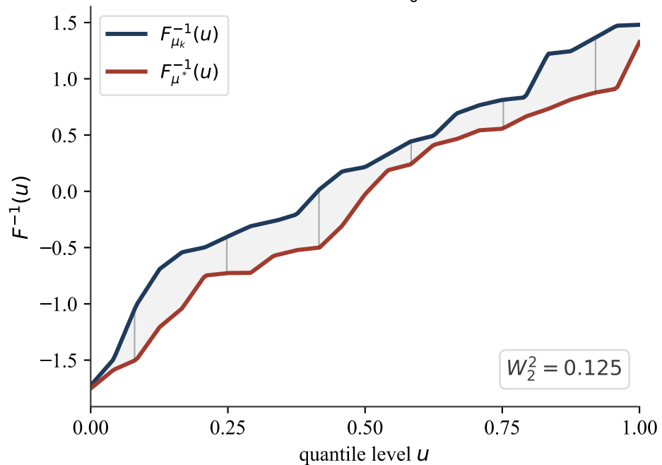
(b) Quantile functions — W_2^2 = \int_0^1 |F_{\mu_k}^{-1} - F_{\mu^*}^{-1}|^2 du
