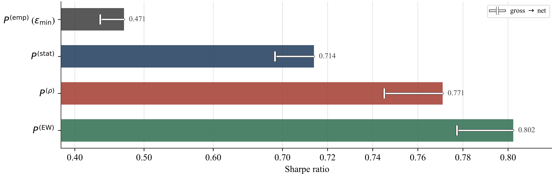
Sharpe ratio across the DRO continuum
