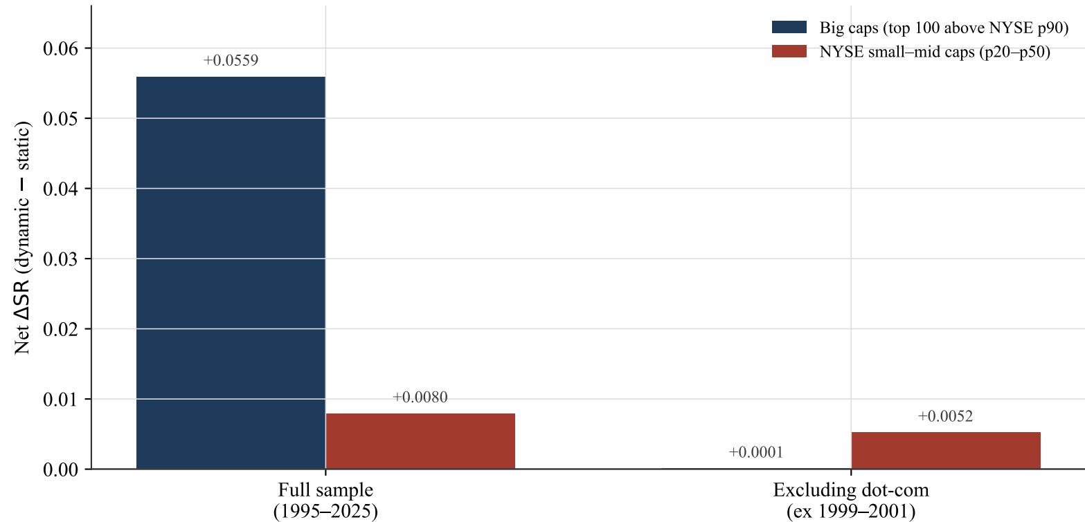
Timing gain by capitalization universe
