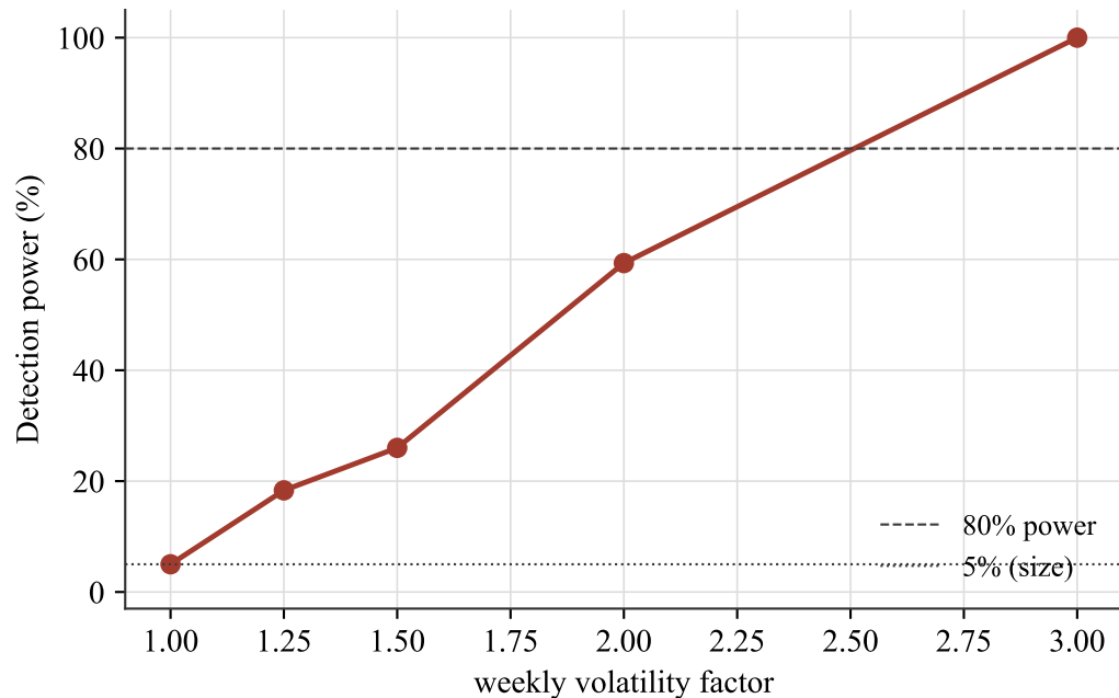
Volatility misalignment
