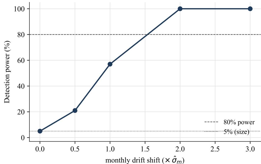
Drift misalignment
