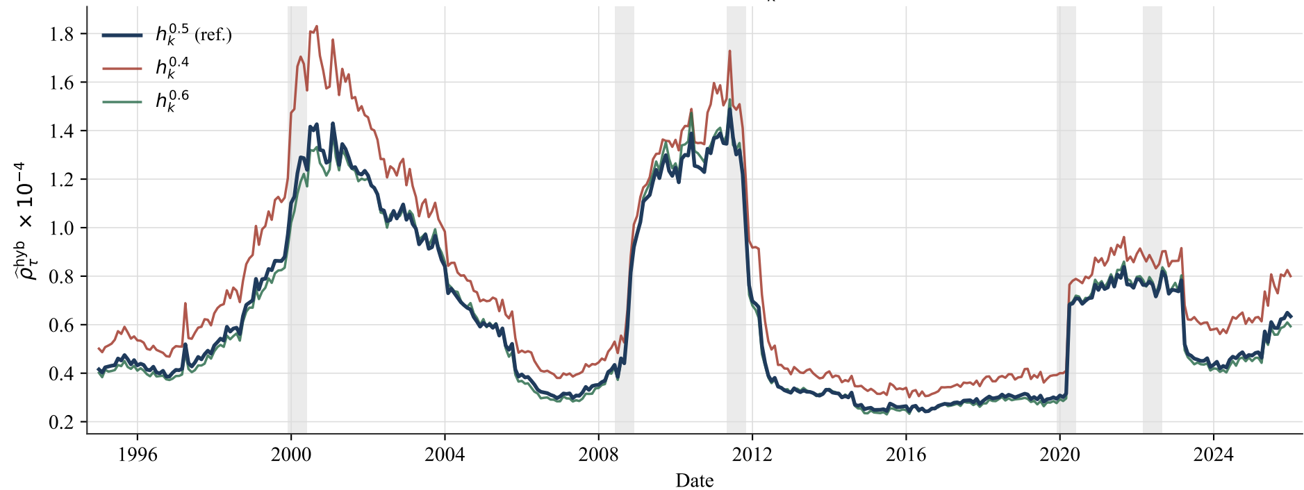
Robustness: scaling exponent h_k^H (1995-2025)
