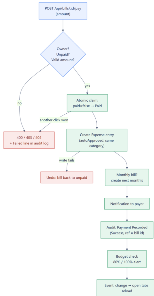
Figure 24. Bill payment cascade (I2)
