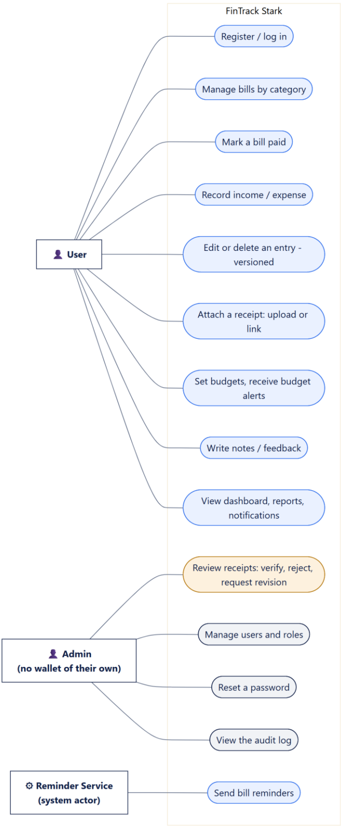
Figure 4. Use-Case Diagram: functions per role
