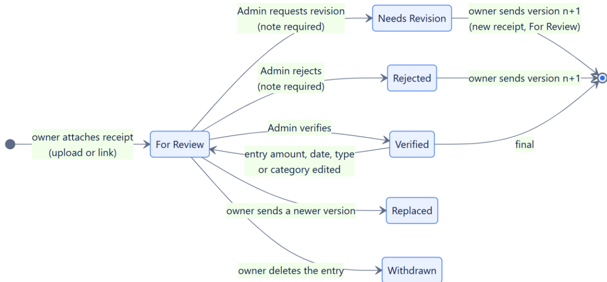
Figure 25. Receipt status life cycle (I3)
