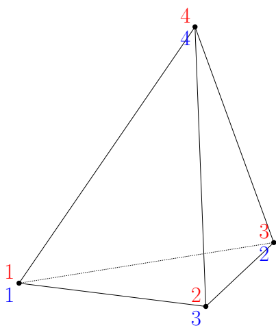
TETRA4
