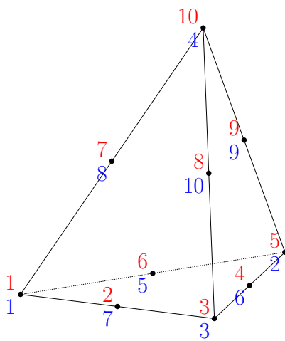
TETRA10
