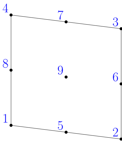
QUAD9
