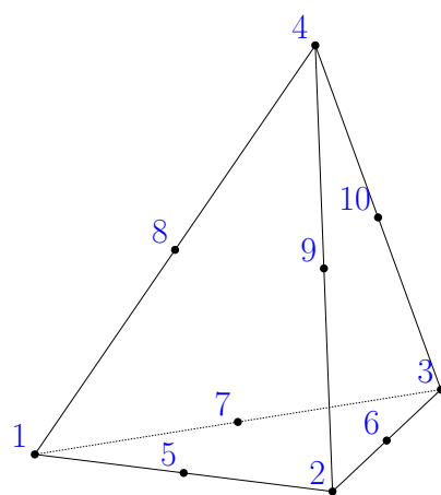
TETRA10
