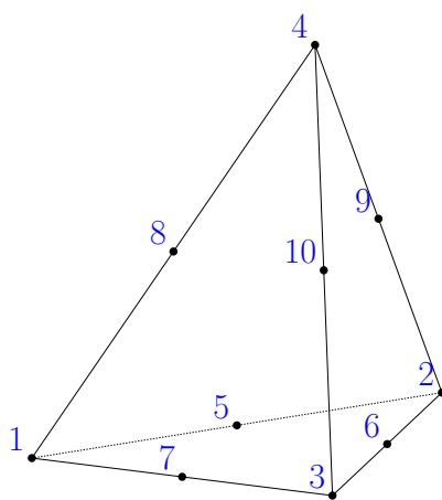
TETRA10
