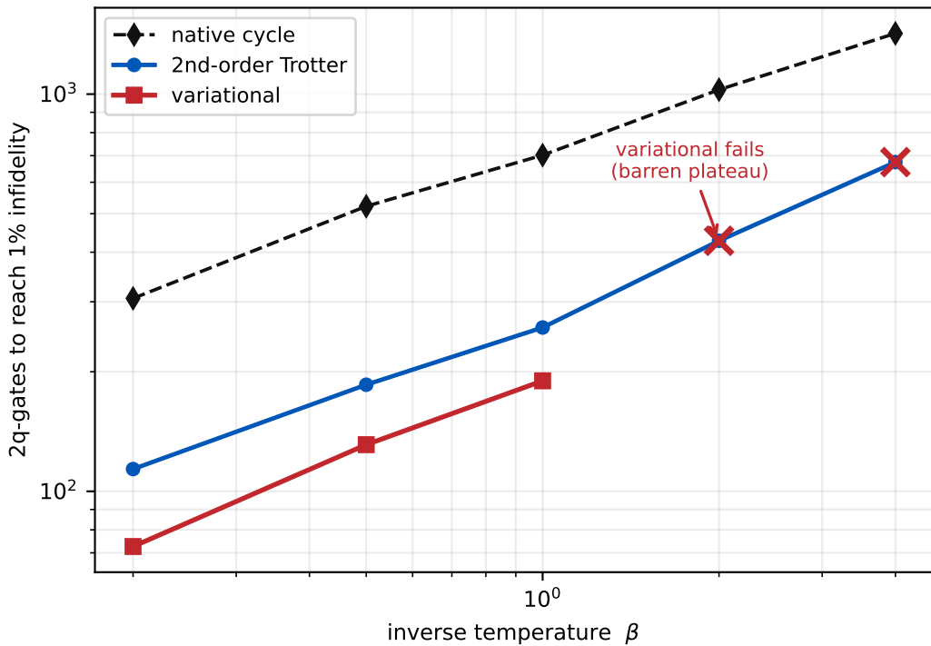
Compression vs temperature
