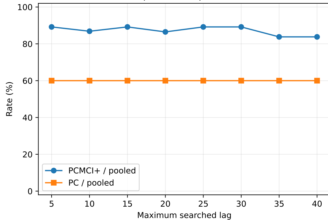
Contemporaneous orientation precision (operational, pooled)
