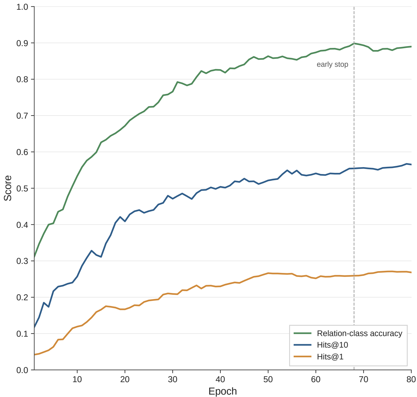
Validation Accuracy and Ranking Metrics
